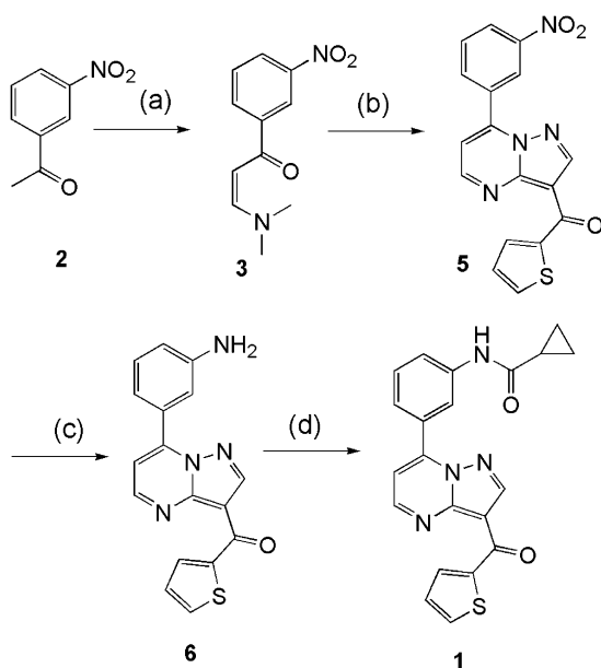
Scheme 1. Reagents and conditions: (a) \text{Me}_2\text{NCH(OMe)}_2 , reflux, 18 h, 89%; (b) 4 , acetic acid, reflux, 82%; (c) \text{Fe} , \text{NH}_4\text{Cl} , \text{MeOH} , \text{H}_2\text{O} , 61%; (d) cyclopropyl carbonyl chloride, pyridine, 0 °C to rt, 6 h, 82%.
