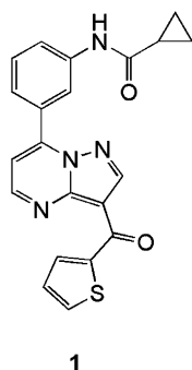
Figure 1. High throughput screen lead for identification of p21 chemoselective agent.
