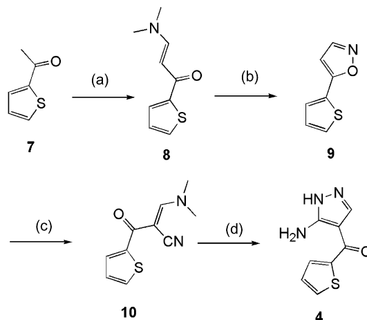
Scheme 2. Reagents and conditions: (a) \text{Me}_2\text{NCH(OMe)}_2 , reflux, 18 h, 92%; (b) \text{NH}_2\text{OH}\cdot\text{HCl} , reflux, 3 h, 65%; (c) \text{Me}_2\text{NCH(OMe)}_2 , reflux, 18 h, 74%; (d) \text{NH}_2\text{NH}_2\cdot\text{H}_2\text{O} , 60%.
