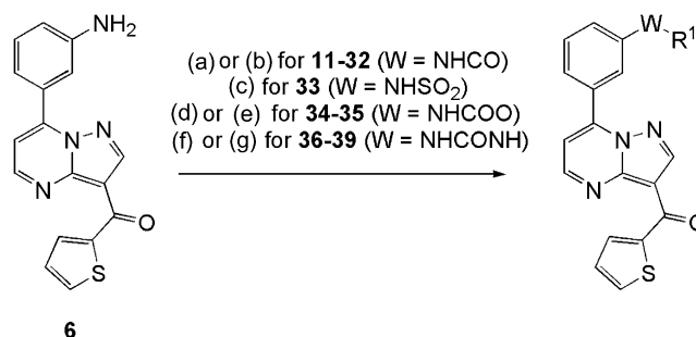
Scheme 3. Parallel synthesis. Reagents and conditions: (a) \text{R}^1\text{COCl} , pyridine, 0 °C to rt, 6 h; (b) \text{R}^1\text{COOH} , EDCI, HOBT, \text{Et}_3\text{N} , DMF, rt, 12 h; (c) \text{R}^1\text{SO}_2\text{Cl} , pyridine, 0 °C to rt, 6 h; (d) \text{R}^1\text{OCOCl} , pyridine, 0 °C to rt, 6 h; (e) 1 : (4- \text{NO}_2\text{Ph} ) \text{OCOCl} , pyridine, 0 °C to rt, 3 h, 2: \text{R}^1\text{OH} , rt, 18 h; (f) \text{R}^1\text{NCO} , pyridine, 0 °C to rt, 6 h; (g) 1 : (4- \text{NO}_2\text{Ph} ) \text{OCOCl} , pyridine, 0 °C to rt, 3 h, 2: \text{R}^1\text{NH}_2 , rt, 18 h.
